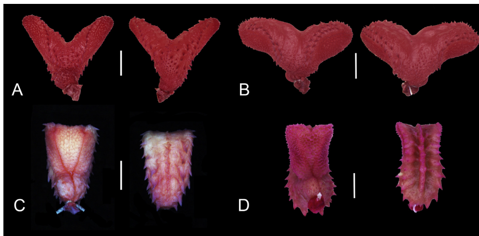
Fig. 12. Hemipenial morphology of Tropidodryadini and Xenoxobelis showing the asulcated and sulcated views. (A) MNRJ 13263 Tropidodryas serra from Cananéia, São Paulo, Brazil. (B) MNRJ 7406 Tropidodryas striaticeps from Lima Duarte, Minas Gerais, Brazil. (C) MNRJ 3876 Xenoxobelis argenteus from Presidente Figueiredo, Amazonas, Brazil. (D) MNRJ 26161 Xenoxobelis boulengeri from Boca do Acre, Amazonas, Brazil.
