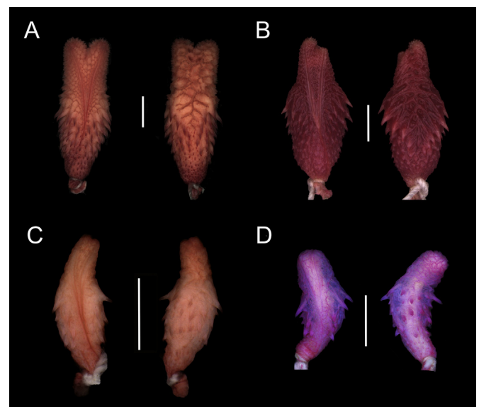
Fig. 5. Hemipenial morphology of all Chlorosoma species showing asulcate and sulcate views (A) MNRJ 23683 Chlorosoma lateiceps from Linhares, Espírito Santo, Brazil. (B) MNRJ 26648 Chlorosoma viridissimum from Rio Branco, Acre, Brazil. (C) UFAC-RB 421 Chlorosoma dunupyana paratype from type locality. (D) CORBIDI 19094 Chlorosoma dunupyana paratype from La Convención, Cusco, Peru.
