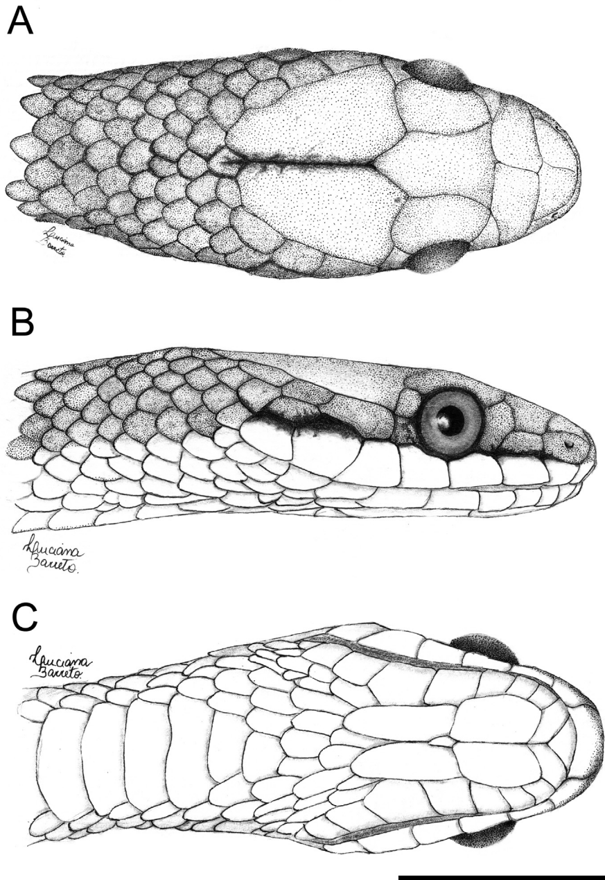
Fig. 8. Dorsal (A), lateral (B) and ventral views (C) of the holotype of Chlorosoma dunupyana sp. nov. (UFAC-RB 345) from Parque Zoobotânico, Rio Branco, Acre, Brazil.
